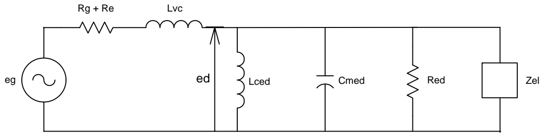
Figure 8.3 : Electrical Equivalent Circuit for a Back Loaded Horn Speaker
