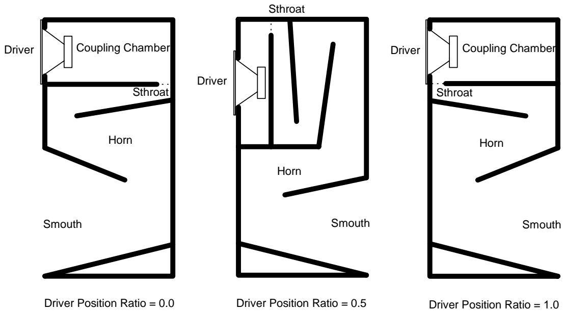
Figure 8.1 : Back Loaded Horn Geometry
