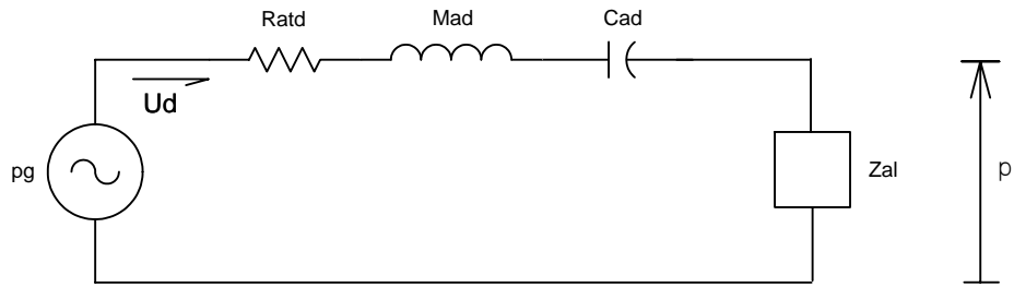
Figure 8.2 : Acoustic Equivalent Circuit for a Back Loaded Horn Speaker
